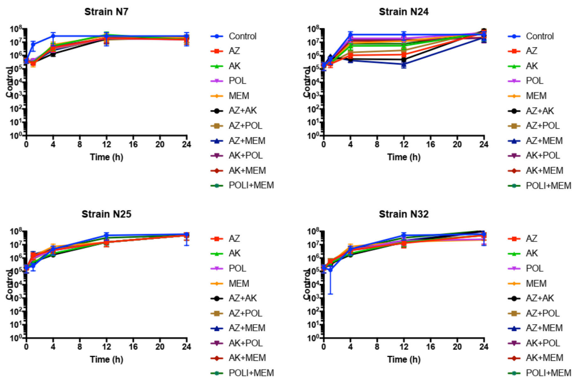
Fig. 1. Time-kill curve of four isolates of S. marcescens exposed to different antibiotics and combinations. The blue line is the positive control. AZ, Aztreonam; AK, Amikacin; POL, Polymyxin; MEM, Meropenem.
